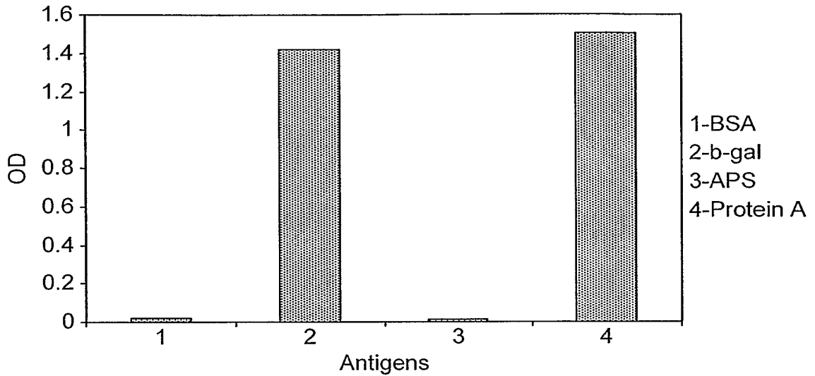
Soluble ScFv ELISA of K8V K /dummy V H clone
